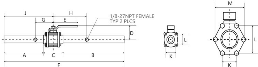
Gauge Port Design
